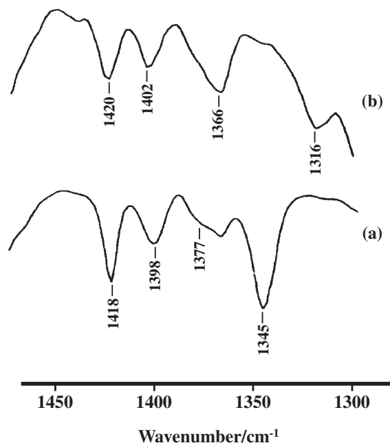
Figure 2. The IR spectra of SDHS·1.2H 2 O (a) and SDHS·2.3H 2 O (b) in the region 1300–1450 cm −1 .
