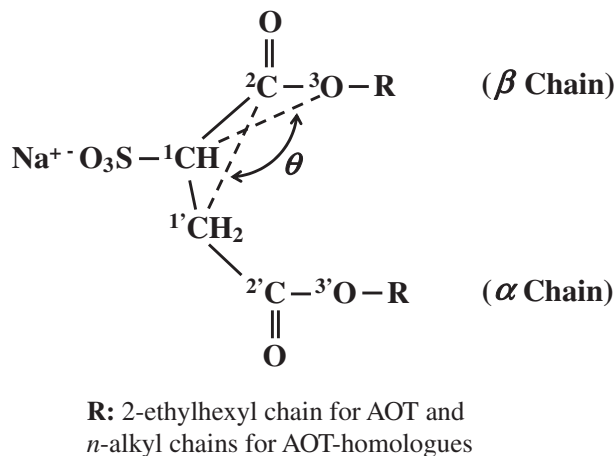
Scheme 1. Atomic numbering of the molecular formula of the succinate segment of AOT and its homologs. \theta denotes the torsion angle of the 1 C– 1 C– 2 C(=O)– 3 O skeleton.
